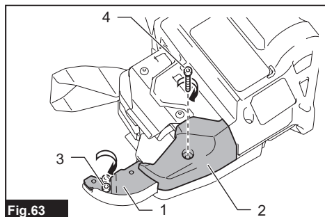
Fig.63 ► 1. Wire guide B 2. Contact plate cover 3. Bolt A 4. Bolt B
