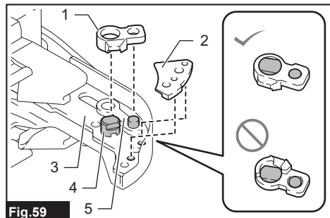
Fig.59 ► 1. Cutter B 2. Top plate 3. Arm plate A 4. Cutter A 5. Link arm A
